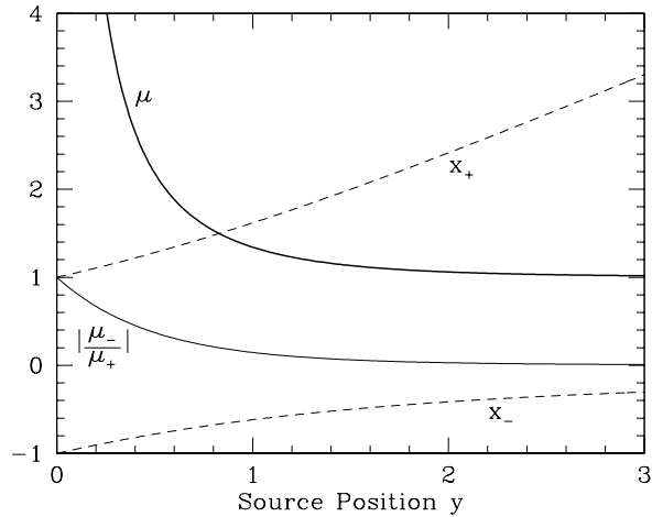
Fig. 1. Total magnification \mu , normalized image positions x_{\pm} , and ratio of image magnifications for a point lens as a function of the normalized source position y (Figure courtesy Penny Sackett)
