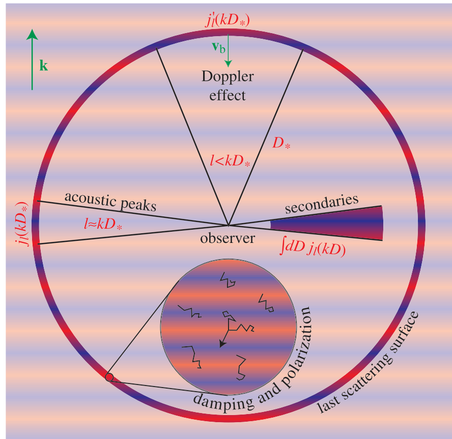
Plate 3: Integral approach. CMB anisotropies can be thought of as the line-of-sight projection of various sources of plane wave temperature and polarization fluctuations: the acoustic effective temperature and velocity or Doppler effect (see §3.8), the quadrupole sources of polarization (see §3.7) and secondary sources (see §4.2, §4.3). Secondary contributions differ in that the region over which they contribute is thick compared with the last scattering surface at recombination and the typical wavelength of a perturbation.
