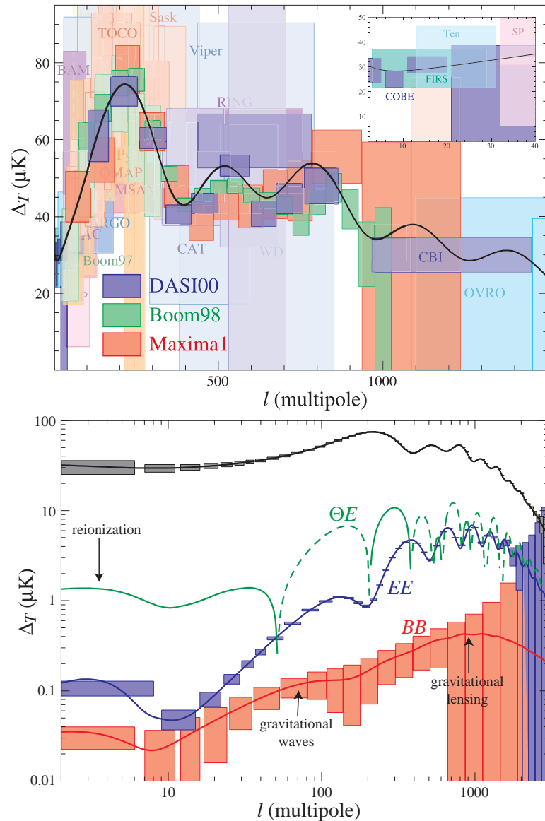
Plate 1: Top: temperature anisotropy data with boxes representing 1\text{-}\sigma errors and approximate l -bandwidth. Bottom: temperature and polarization spectra for \Omega_{\text{tot}} = 1 , \Omega_\Lambda = 2/3 , \Omega_b h^2 = 0.02 , \Omega_m h^2 = 0.16 , n = 1 , z_{\text{ri}} = 7 , E_i = 2.2 \times 10^{16} GeV. Dashed lines represent negative cross correlation and boxes represent the statistical errors of the Planck satellite.
