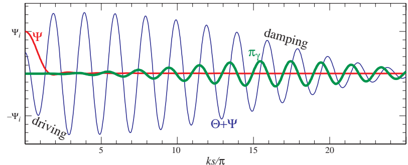
Figure 3: Radiation driving and diffusion damping. The decay of the potential \Psi drives the oscillator in the radiation dominated epoch. Diffusion generates viscosity \pi_\gamma , i.e. a quadrupole moment in the temperature, which damps oscillations and generates polarization. Plotted here is the numerical solution to Equation (18) and Equation (19) for a mode with wavelength much smaller than the sound horizon at decoupling, ks_* \gg 1 .
