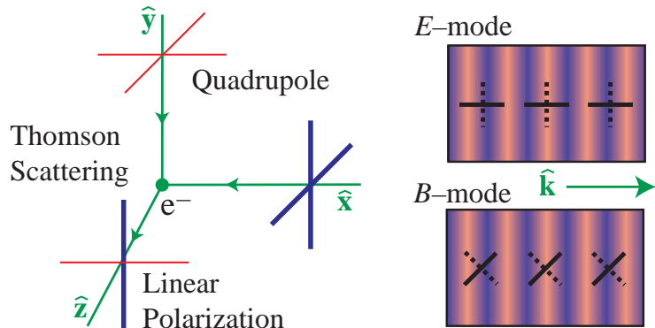
Plate 2: Polarization generation and classification. Left: Thomson scattering of quadrupole temperature anisotropies (depicted here in the \hat{x}-\hat{y} plane) generates linear polarization. Right: Polarization in the \hat{x}-\hat{y} plane along the outgoing \hat{z} axis. The component of the polarization that is parallel or perpendicular to the wavevector \mathbf{k} is called the E -mode and the one at 45° angles is called the B -mode.
