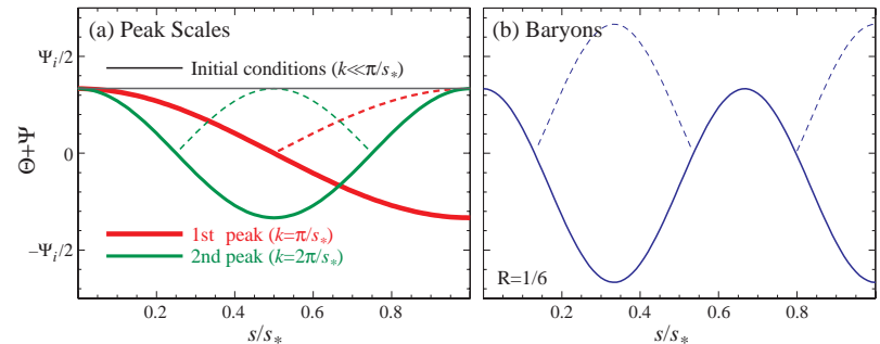
Figure 1: Idealized acoustic oscillations. (a) Peak scales: the wavemode that completes half an oscillation by recombination sets the physical scale of the first peak. Both minima and maxima correspond to peaks in power (dashed lines, absolute value) and so higher peaks are integral multiples of this scale with equal height. Plotted here is the idealization of Equation (15) (constant potentials, no baryon loading). (b) Baryon loading. Baryon loading boosts the amplitudes of every other oscillation. Plotted here is the idealization of Equation (16) (constant potentials and baryon loading R = 1/6 ) for the third peak.
