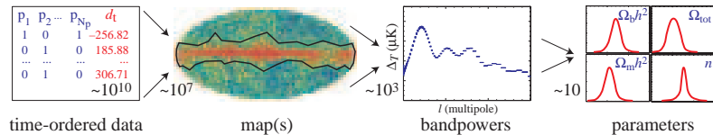
Figure 5: Data pipeline and radical compression. Map are constructed for each frequency channel from the data timestreams, combined and cleaned of foreground contamination by spatial (represented here by excising the galaxy) and frequency information. Bandpowers are extracted from the maps and cosmological parameters from the bandpowers. Each step involves a substantial reduction in the number of parameters needed to describe the data, from potentially 10^{10} \rightarrow 10 for the Planck satellite.
