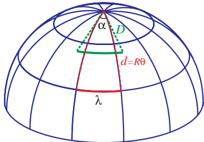
Figure 2: Angular diameter distance. In a closed universe, objects are further than they appear to be from Euclidean (flat) expectations corresponding to the difference between coordinate distance d and angular diameter distance D . Consequently, at a fixed coordinate distance, a given angle corresponds to a smaller spatial scale in a closed universe. Acoustic peaks therefore appear at larger angles or lower \ell in a closed universe. The converse is true for an open universe.
