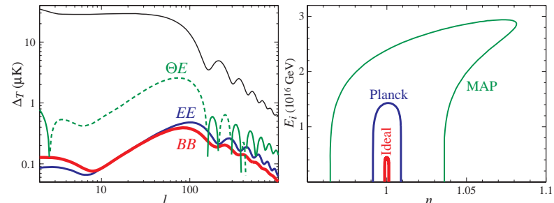
Figure 4: Gravitational waves and the energy scale of inflation E_i . Left: temperature and polarization spectra from an initial scale invariant gravitational wave spectrum with power \propto E_i^4 = (4 \times 10^{16} \text{ GeV})^4 . Right: 95% confidence upper limits statistically achievable on E_i and the scalar tilt n by the MAP and Planck satellites as well as an ideal experiment out to l = 3000 in the presence of gravitational lensing B -modes.
