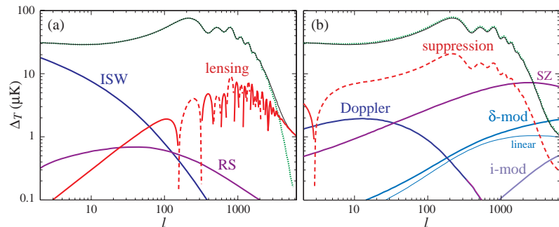
Plate 5: Secondary anisotropies. (a) Gravitational secondaries: ISW, lensing and Rees-Sciama (moving halo) effects. (b) Scattering secondaries: Doppler, density ( \delta ) and ionization (i) modulated Doppler, and the SZ effects. Curves and model are described in the text.
