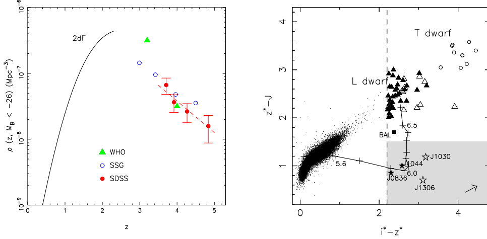
Fig. 1.3. Left: The space density of quasars with M_B < -26 mag as a function of redshift for the 2dF, SDSS, SSG, and WHO surveys (Fan et al. 2001b). Right: The z^* - J versus i^* - z^* diagram for the SDSS, showing how the infrared J band enables the separation of z > 5.8 quasars from the numerous L and T dwarfs (Fan et al. 2001c).
