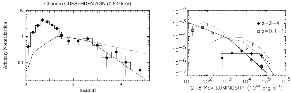
Fig. 1.5. Left : The redshift distribution for 243 AGNs in the Chandra Deep Field South and Hubble Deep Field North surveys, from Hasinger (2003), compared to population synthesis models by Gilli et al. (2001), where the dashed line is for the redshift decline of SSG for z > 2.7 and the dotted line is for a constant space density for z > 1.5 . Note the observed excess of objects at z < 1 . Right : Luminosity functions derived from Chandra , ROSAT , and ASCA surveys by Cowie et al. (2003), based on their redshift measurements and estimates. Note that the values for sources with z < 1 and L_X < 10^{43} erg s -1 are well above those for the 2 < z < 4 objects.
