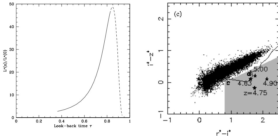
Fig. 1.2. Left : A linear plot of the characteristic luminosity of quasars from the 2dF (Boyle et al. 2000) and SSG samples versus look-back time, for the luminosity evolution model. Right : A i^* - z^* versus r^* - i^* plot of SDSS data, showing the stellar locus (black area and points) and how quasars with 4.6 < z < 5.0 separate from the stellar locus because of the presence of Ly \alpha emission in the i^* band and of Ly \alpha forest absorption in the r^* band (Fan et al. 1999).
