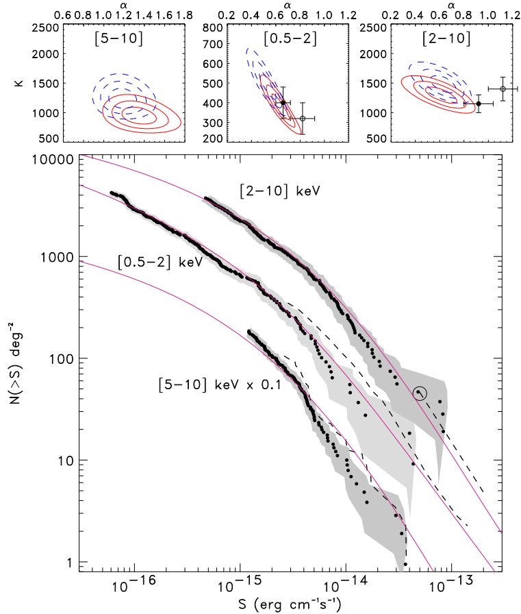
Fig. 1.4. The log N -log S data for the Chandra Deep Field South survey for three different energy bands. The upper boxes show the fits for the normalization constant, \kappa , and slope, \alpha , of the faint end of the data (Rosati et al. 2002).
