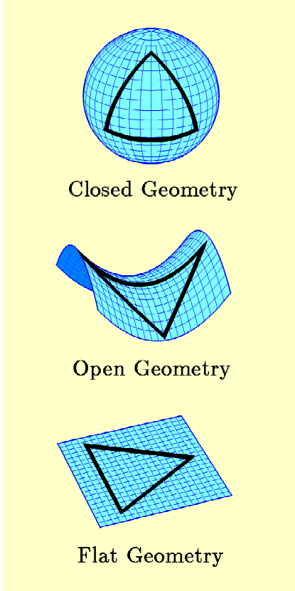
FIG. 2: According to general relativity, spacetime may be warped or curved, depending on the density of mass-energy. Inflation predicts that our observable universe should be spatially flat to very high accuracy.
