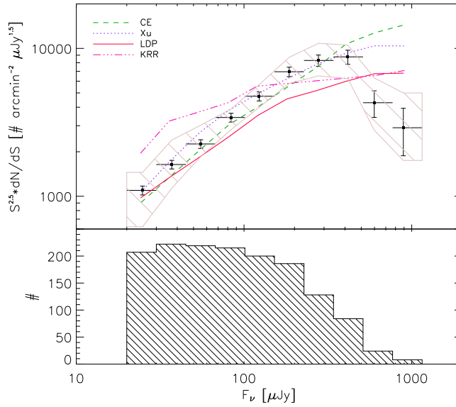
Figure 17. Completeness corrected galaxy counts in the MIPS 24 \mu\text{m} channel from Spitzer observations of the ELAIS-N1 field (from Chary et al. 2004). The error bars reflect the Poissonian uncertainty. The horizontal bars represent the minimum and maximum flux density in that bin. The lines show four models for 24 \mu\text{m} counts: King & Rowan-Robinson (2003, KRR), Xu et al. (2001, Xu), Chary & Elbaz (2001, CE), Lagache, Dole & Puget (2003, LDP). The symbols are plotted at the average of the flux densities of the detected sources in that bin for the data while the lines are plotted at the counts-weighted flux average for the models. The lower plot in the figure shows the histogram of the actual number of sources detected in each flux bin without any completeness correction.
