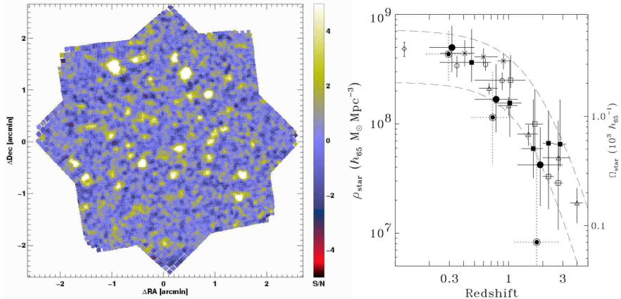
Figure 3. (left) ISOCAM 6.75 \mu\text{m} image of the SSA13 field (Fig.2 from Sato et al. 2003, 23 hour observation). This image reaches an 80 % completeness limit of 16 \mu\text{Jy} in the central 7 \text{ arcmin}^2 region. North is top and east to the left in J2000. The center is (RA, Dec) = ( 13^{\text{h}} 12^{\text{m}} 26^{\text{s}}, 42^{\circ} 44' 24''.8 ). The map shows signal-to-noise ratio (S/N) per 0.6 arcsec sub-pixel. The signal is an average, weighted by the inverse of the assigned variance, and the noise is a normalized standard deviation. (right) Stellar mass density in the universe as a function of redshift (Fig.13 from Sato et al. 2004). The right axis shows densities normalized to the critical density of the universe. The contributions of the 6.75 \mu\text{m} galaxies are shown with solid and double circles for the “combined” (including photometric redshifts) and purely spectroscopic samples, respectively. The double circles are plotted at slightly lower redshifts. The horizontal bars represent the redshift ranges of the bins and the vertical bars show one sigma errors, taking account of Poisson noise and uncertainties in stellar mass and V_{\text{max}} . Several other estimates are overlaid (see Sato et al. 2004 for references). The empty/solid squares and the diamond are obtained from full integration of a Schechter fit to their respective luminosity or stellar mass function at each redshift bin. The X marks and the empty circles are quasi-fully integrated values with a finite integration range from 10 L^* to 1/20 L^* , and 10.5 < \log(M_{\text{star}}[h_{65}^{-2} M_{\odot}]) < 11.6 , respectively. The triangles are simply summed values of the detected sources. The two dashed curves are deduced by integrating the star formation rate density in the universe, which is derived from the UV luminosity density as a function of redshift (Cole et al. 2001). The upper curve is an extinction corrected case for E(B - V) = 0.15 , and the lower one has no dust correction.
