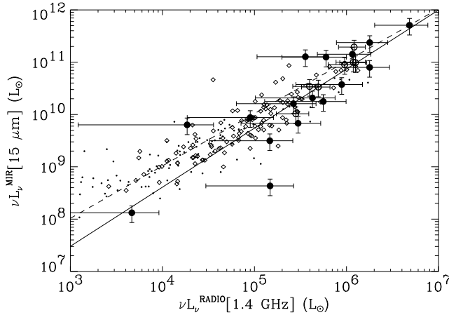
Figure 10. 15 \mu\text{m} versus radio continuum (1.4 GHz) rest-frame luminosities. Small filled dots: sample of 109 local galaxies from ISOCAM and NVSS. Filled dots with error bars: 17 HDFN galaxies ( z \sim 0.7 , radio from VLA or WSRT). Open dots with error bars: 7 CFRS-14 galaxies ( z \sim 0.7 , Flores et al. 1999, radio from VLA). Open diamonds: 137 ELAIS galaxies ( z \sim 0-0.4 ).
