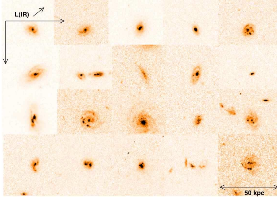
Figure 13. HST-ACS images of LIR galaxies with 11 \leq \log(L_{\text{IR}}/L_{\odot}) \leq 12 (LIRGs) and z \sim 0.7 . The double-headed arrow indicates the physical size of 50 kpc. The IR luminosity increases from left to right and from top to bottom.
