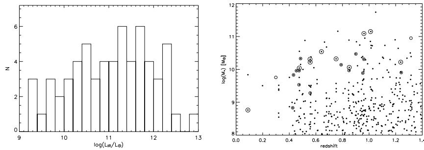
Figure 12. (left) Distribution of the \log(L_{\text{IR}} (8-1000 \mu\text{m})/L_{\odot}) of the HDFN+FF ISOCAM galaxies derived from their 15 \mu\text{m} flux densities. (right) Stellar mass as a function of redshift of field HDFN proper galaxies (dark dots) and of ISOCAM galaxies (open circles). All stellar masses were derived using multi-bands SED modelling by Dickinson et al. (2003).
