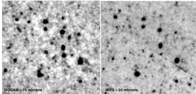
Figure 18. ISOCAM 15 \mu\text{m} image (left) of the Ultra-Deep Survey in the Marano FIRBACK field (depth 140 \mu\text{Jy} , 80% completeness) versus Spitzer MIPS-24 \mu\text{m} image (right; depth 110 \mu\text{Jy} , 80% completeness). The crosses identify 16 galaxies detected at 15 and 24 \mu\text{m} for which VLT-FORS2 spectra were obtained and which SEDs were fitted in Elbaz et al. (2004).
