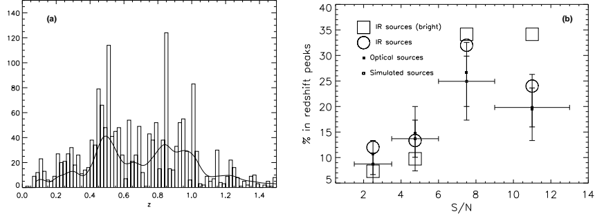
Figure 14. (a) Redshift distribution of field galaxies in the GOODS field. The continuous line is the smoothed distribution with a window of 15,000 km/s. (b) Differential fraction of sources within redshift peaks (see definition in the text) stronger than N\text{-}\sigma . Small filled squares: fraction of sources in peaks for the whole optical catalog of 930 field galaxies (Wirth et al. 2004). Small open squares: median of the fraction of sources in redshift peaks for a series of Monte Carlo simulations of a sub-sample of the field galaxies corresponding to the same number of galaxies as in the ISOCAM catalog and within the same range of redshifts and optical-near IR magnitudes. Error bars contain 68 and 90% of the simulations. Large Open Circles: total sample of ISOCAM galaxies (75 sources with spectroscopic redshifts and optical-near IR magnitudes). Large open squares: sub-sample of ISOCAM galaxies above the completeness limit of 0.1 mJy (41 sources).
