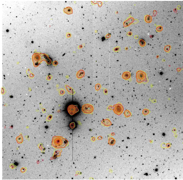
Figure 7. ISOCAM 15\ \mu\text{m} contours overlaid on the VLT-FORS2 image ( 7' \times 7' , R-band) of the Marano FIRBACK Ultra Deep Survey (UDSF). The LARI (light contours, yellow on screen, grey on paper) and PRETI (dark contours, red on screen) detect the same objects.
