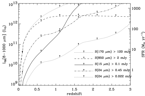
Figure 2. Sensitivity limits of ISOCAM ( 15 \mu\text{m} , 0.1 \text{ mJy} ), ISOPHOT ( 170 \mu\text{m} , 120 \text{ mJy} ), SCUBA ( 850 \mu\text{m} , 2 \text{ mJy} ) and Spitzer ( 24 \mu\text{m} , 0.45 \text{ mJy} and 0.022 \text{ mJy} ) corresponding to the expected detection limits of the SWIRE and GOODS Legacy Programs). This figure was generated assuming that distant galaxies SEDs are similar to local ones. We used the library of template SEDs constructed by Chary & Elbaz (2001).
