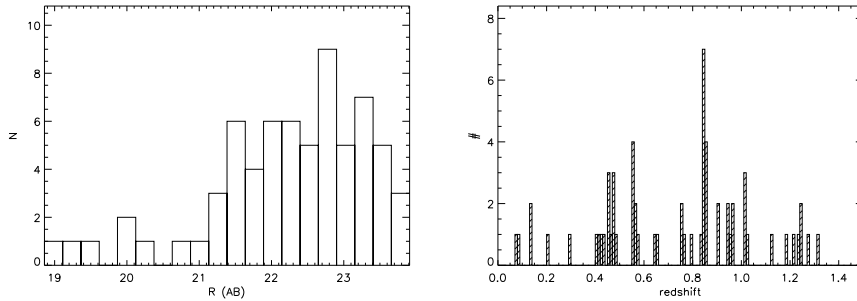
Figure 11. (left) Histogram of the R(AB) magnitudes of the 15 \mu\text{m} ISOCAM galaxies detected in the HDFN+FF (revised catalog of Aussel et al. down to \sim 30 \mu\text{Jy} ). (right) Redshift distribution of the HDFN+FF ISOCAM galaxies.
