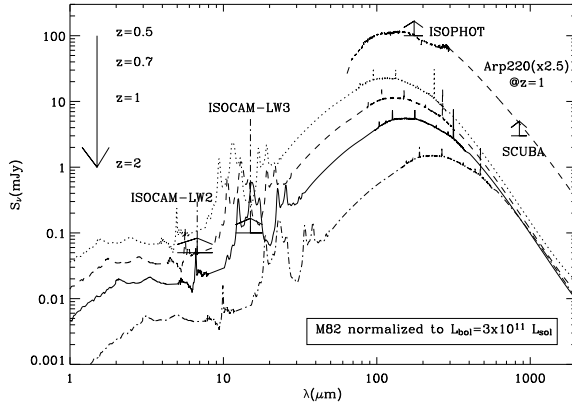
Figure 1. Effect of the k-correction on the detection of distant LIRGs and ULIRGs by ISOCAM, ISOPHOT and SCUBA. Only ISOCAM at 15 \mu\text{m} can detect LIRGs up to z \sim 1 , while ISOPHOT and SCUBA are sensitive to distant ULIRGs of a few 10^{12} L_{\odot} .
