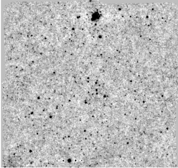
Figure 6. ISOCAM 15\ \mu\text{m} image of the Marano FIRBACK Deep Survey (DSF) from the IGTES (Elbaz et al. 1999, and in prep.). Data reduction with PRETI.
