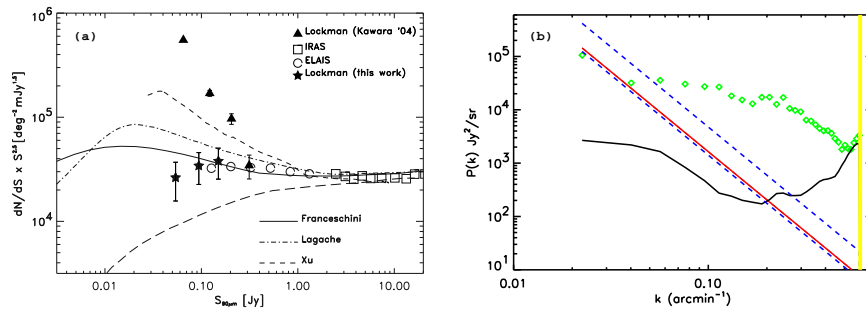
Figure 4. (a) Differential 90 \mu\text{m} counts dN/dS normalized to the Euclidean law ( N \propto S^{-2.5} ) (extracted from Rodighiero & Franceschini 2004). Results compared with those from the preliminary analysis of the ISOPHOT ELAIS survey (Efstathiou et al. 2000, open circles) and with those from Kawara et al. (2004, filled triangles). The long-dashed line shows the expected contribution of non-evolving spirals as in the model of Franceschini et al. (2001). (b) Fluctuations of the CIB in a power spectrum analysis of the FIRBACK/ELAIS N2 field at 170 microns by Puget & Lagache (2000). Observed power spectrum: diamond; straight continuous line: the best fit cirrus power spectrum; dash line: cirrus power spectrum deduced from Miville-Deschênes et al. (2002); continuous curve: detector noise.
