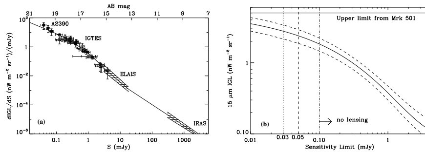
Figure 8. a) Differential contribution to the 15 \mu m Integrated Galaxy Light as a function of flux density and AB magnitude. The plain line is a fit to the data: Abell 2390 (Altieri et al. 1999), the ISOCAM Guaranteed Time Extragalactic Surveys (IGTES, Elbaz et al. 1999), the European Large Area Infrared Survey (ELAIS, Serjeant et al. 2000) and the IRAS all sky survey (Rush, Malkan & Spinoglio 1993). b) Contribution of ISOCAM galaxies to the 15 \mu m extragalactic background light (EBL), i.e. 15 \mu m Integrated Galaxy Light (IGL), as a function of sensitivity or AB magnitude ( AB = -2.5 \log(S_{mJy}) + 16.4 ). The plain line is the integral of the fit to dIGL/dS (Fig.a). The dashed lines correspond to 1- \sigma error bars obtained by fitting the 1- \sigma upper and lower limits of dIGL/dS .
