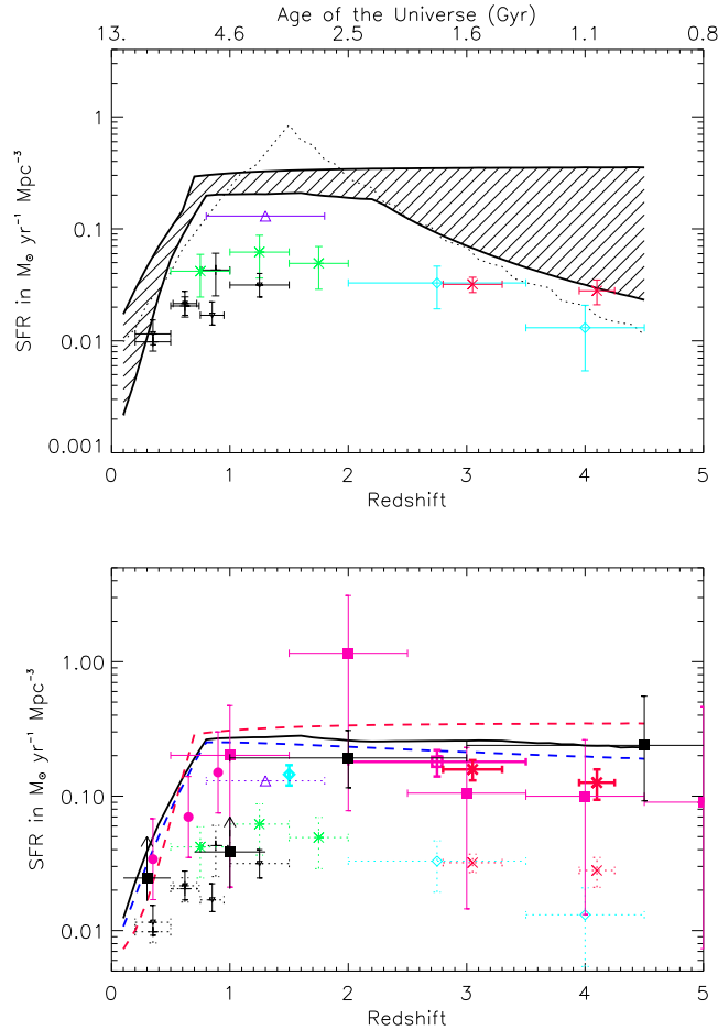
Figure 15. Star Formation Rate from Chary & Elbaz (2001). Upper panel: min and max range from their model, and observed UV/opt data; dots represent Xu et al. (2001) model. Lower panel: 3 different evolution scenarios from their model and data corrected for extinction. Line: pure luminosity; upper dash: pure density; lower dash: luminosity+density.
