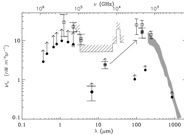
Figure 16. Integrated Galaxy Light (IGL, filled dots) and Extragalactic Background Light (EBL, open squares, grey area) from the UV to sub-millimeter (from Elbaz et al. 2002). EBL measurements from COBE: 200-1500 \mu\text{m} EBL from COBE-FIRAS (grey area, Lagache et al. 1999), 1.25, 2.2, 3.5, 100, 140 \mu\text{m} EBL from COBE-DIRBE (open squares). IGL in the U,B,V,I,J,H,K bands from Madau & Pozzetti (2000). The upper end of the arrows indicate the revised values suggested by Bernstein et al. (2001, factor two higher). 6.75 \mu\text{m} (ISOCAM-LW2 filter) IGL from Metcalfe et al. (2003, filled dot with error bar and arrow). Hatched upper limit from Mkn 501 (Stanev & Franceschini 1998). The ISOCAM 15 \mu\text{m} IGL ( 2.4 \pm 0.5 \text{ nW m}^{-2} \text{ sr}^{-1} ) is marked with a star surrounded by a circle. The other star surrounded by a circle is the prediction of the contribution of the 15 \mu\text{m} sources to 140 \mu\text{m} (Elbaz et al. 2002).
