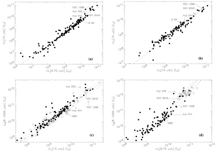
Figure 9. IR luminosity correlations for local galaxies (from Elbaz et al. 2002). a) ISOCAM-LW3 (15 \mu\text{m} ) versus ISOCAM-LW2 (6.75 \mu\text{m} ) luminosities ( \nu L_\nu ) (56 galaxies). b) ISOCAM-LW3 (15 \mu\text{m} ) versus IRAS-12 \mu\text{m} luminosities (45 galaxies). c) L_{\text{IR}}[8-1000 \mu\text{m}] versus ISOCAM-LW3 (15 \mu\text{m} ) luminosity (120 galaxies). d) L_{\text{IR}}[8-1000 \mu\text{m}] versus LW2-6.75 \mu\text{m} luminosities (91 galaxies). Filled dots: galaxies from the ISOCAM guaranteed time (47 galaxies including the open squares). Open dots: 40 galaxies from Rigopoulou et al. (1999). Empty triangles: 4 galaxies from Tran et al. (2001). Galaxies below L_{\text{IR}} \sim 10^{10} L_\odot present a flatter slope and have L_{\text{IR}}/L_B < 1 .
