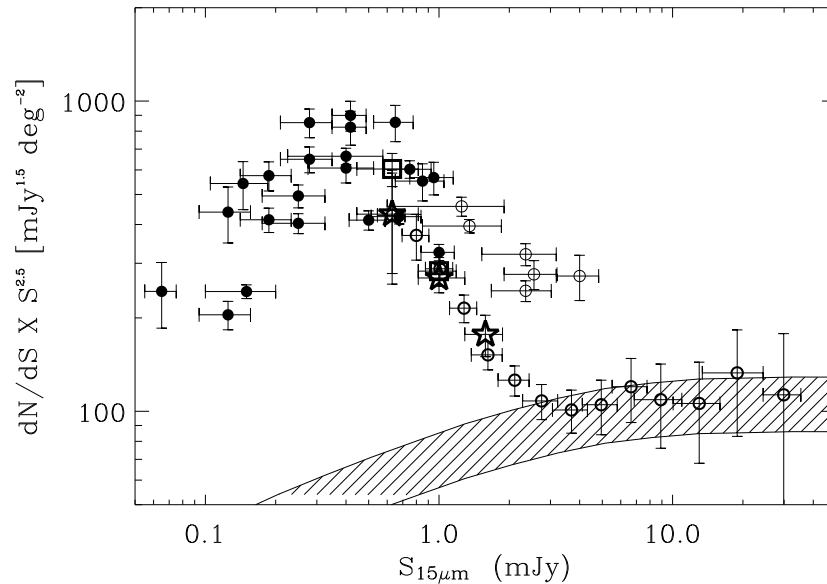
Figure 5. ISOCAM 15\ \mu\text{m} differential counts, with 68% error bars. The counts are normalized to a Euclidean distribution of non-evolving sources, which would have a slope of \alpha = -2.5 in such a universe. This plot is an extension of the Fig.2 from Elbaz et al. (1999) combining the data points from Elbaz et al. (1999), for the ISOCAM Garanteed Time Extragalactic Surveys (IGTES, filled and empty dots for sources below and above 1 mJy respectively, see text), Gruppioni et al. (2003, bold empty circles) for the ELAIS-S1 field, Rodighiero et al. (2004, large open stars) and Fadda et al. (2004, large open squares), for the Shallow and Deep Surveys of the Lockman Hole respectively (analysis of the IGTES data using the “Lari” technique, see Sect. 5). The hatched area materializes the range of possible expectations from models assuming no evolution and normalized to the 15\ \mu\text{m} local luminosity function (LLF) from Fang et al. (1998) and the template SED of M51 (with an assumed uncertainty of \pm 20\% ; this 15\ \mu\text{m} LLF was recently confirmed over a larger sample of local galaxies by H.Aussel, private communication).
