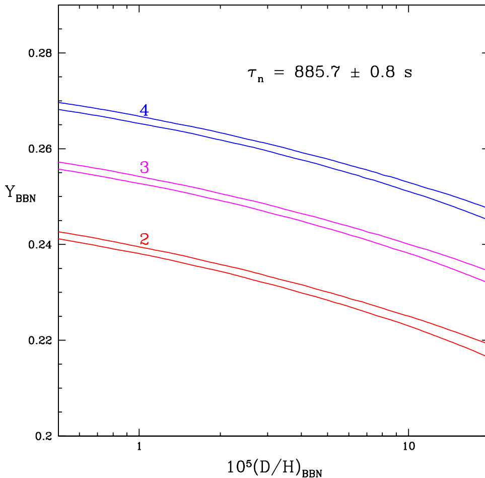
FIGURE 2. The BBN-predicted primordial {}^4\text{He} mass fraction Y as a function of the BBN-predicted primordial Deuterium abundance (by number relative to Hydrogen) for three choices of N_s . The width of the bands represents the theoretical uncertainty, largely due to that of the neutron lifetime \tau_n .
