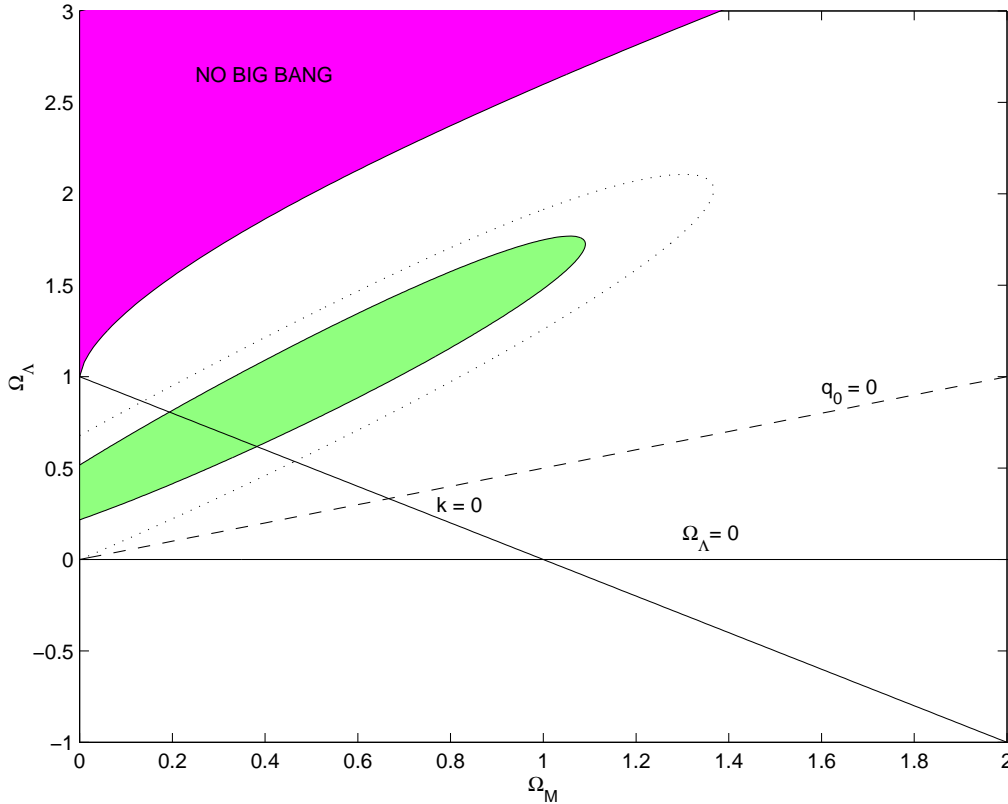
FIGURE 11. The 68% (solid) and 95% (dotted) contours in the \Omega_\Lambda - \Omega_M plane consistent with the SNIa data (see the text). Geometrically flat models lie along the line labelled k = 0 .
