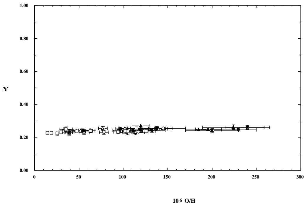
FIGURE 6. The {}^4\text{He} mass fraction, Y , inferred from observations of low-metallicity, extragalactic \text{H II} regions versus the oxygen abundance in those regions.
