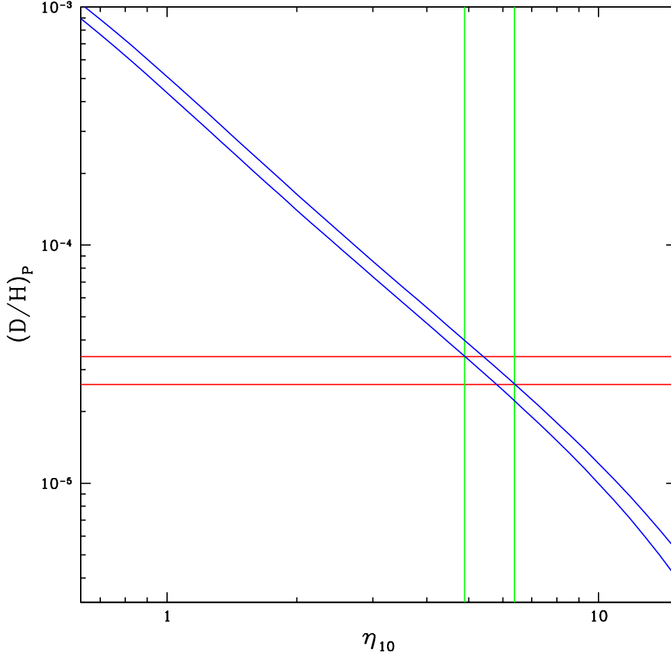
FIGURE 9. The diagonal band is the SBBN-predicted deuterium abundance (by number relative to hydrogen) as a function of the nucleon-to-photon ratio \eta_{10} (the width of the band accounts for the theoretical uncertainties in the SBBN prediction). The horizontal band is the \pm 1\sigma range in the adopted primordial deuterium abundance. The vertical band is, approximately, the corresponding SBBN-predicted \eta range.
